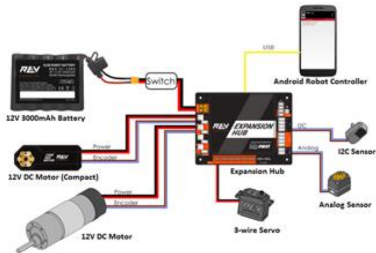
Figure 1: Expansion Hub Configuration
