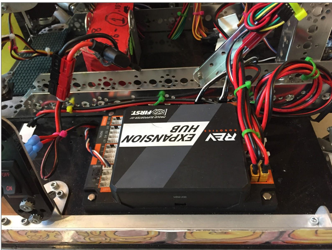
Figure 11: Strain Relief and Wire Restraints
